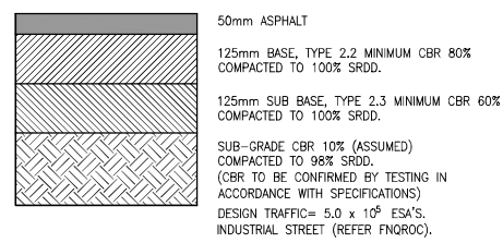
ROAD PAVEMENT DETAIL NOT TO SCALE
