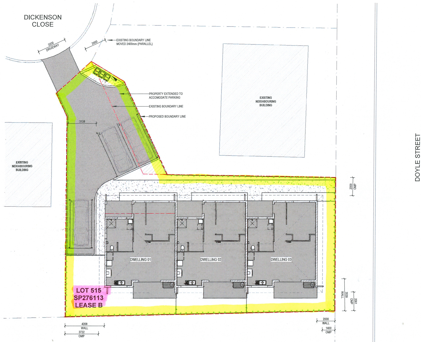
SITE PLAN SCALE 1:100 @ A1
