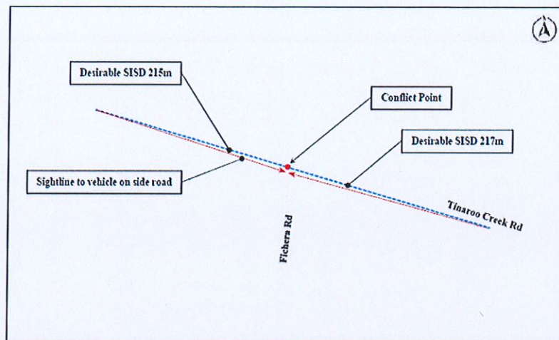
Figure 7.2: Tinaroo Creek Road/Fichera Road Intersection - SISD Assessment
