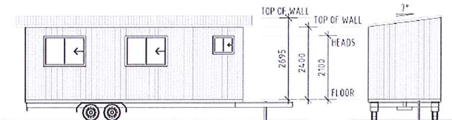
ELEVATIONS SCALE 1:100
