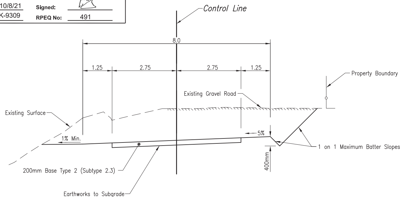
TYPICAL SECTION 00 - 54.659
