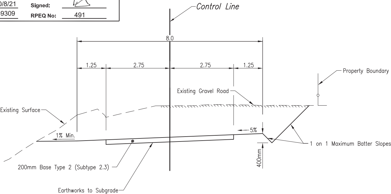
TYPICAL SECTION 00 - 54.659
