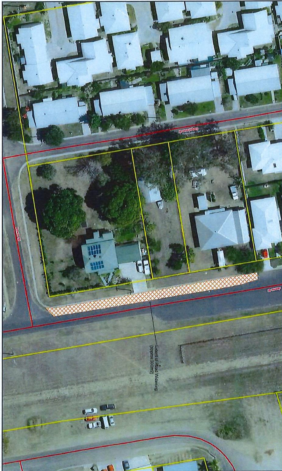
Extent & Detail of Road Widening Works (James Street)
