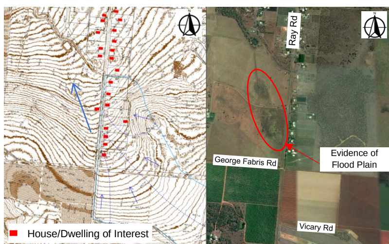
Figure 7: 2018 LiDAR Elevation Data & 2009 Aerial Imagery
